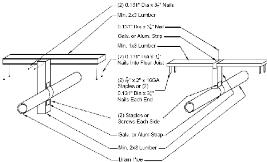
Figure 66. DWV pipe optional support method
