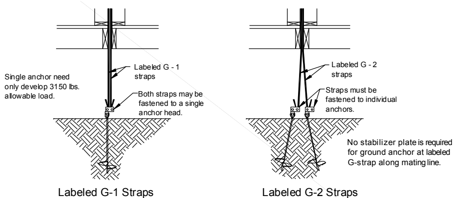
Figure 71. Marriage Line Vertical Anchors
