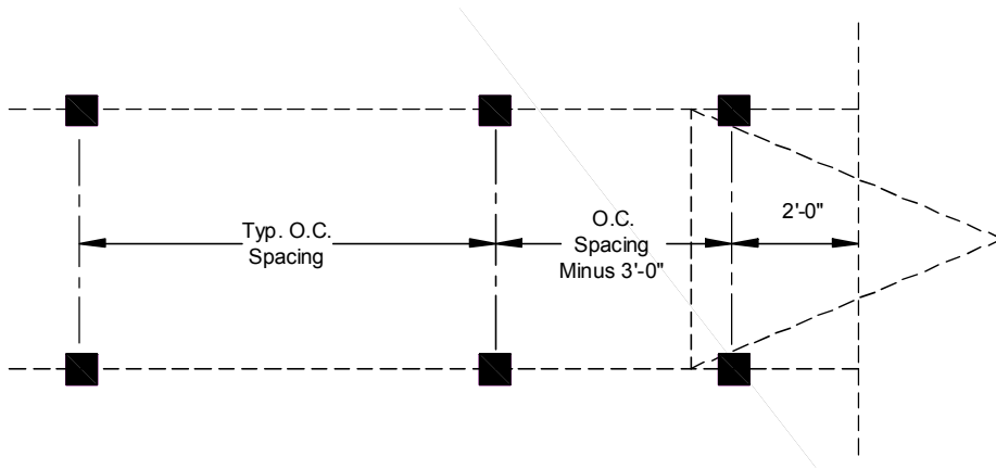
Figure 10. End of beam piering exception
