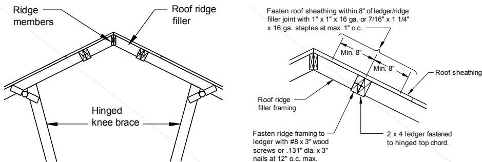
Figure 27. Ridge Filler Option for Hinged Roof
