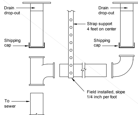
Figure 65. DWV pipe support method
