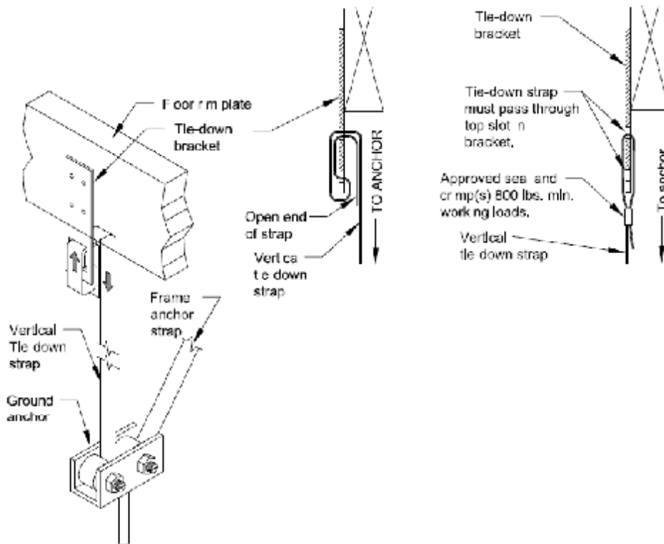
Figure 81. Connecting Sidewall Vertical Strap to Tie-down Bracket
