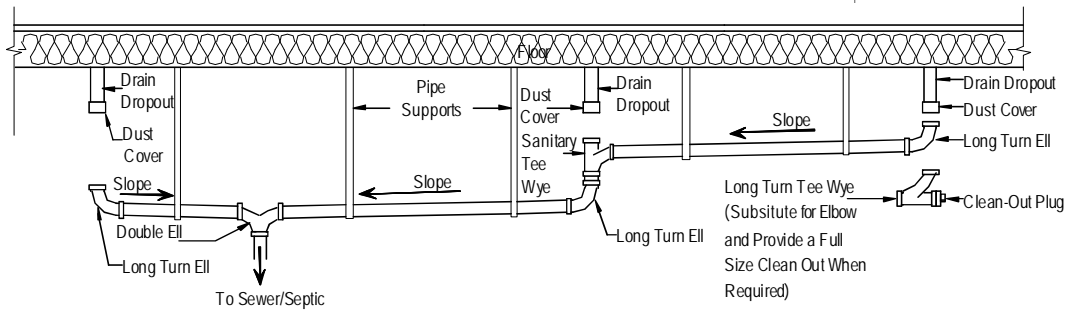
Figure 63. DWV system
