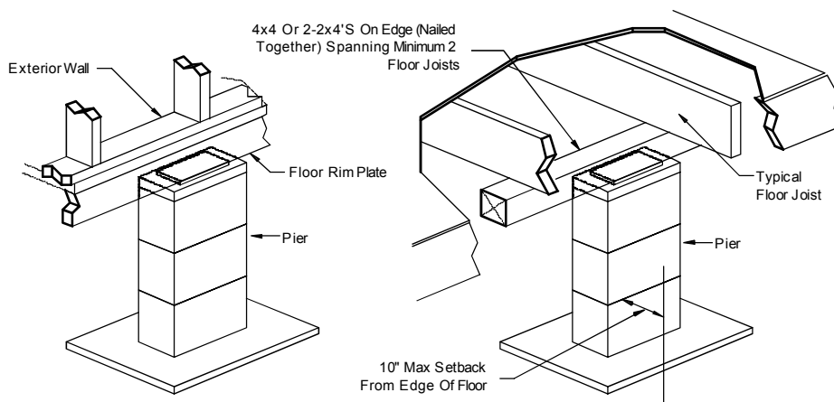
Figure 15. Perimeter supports
